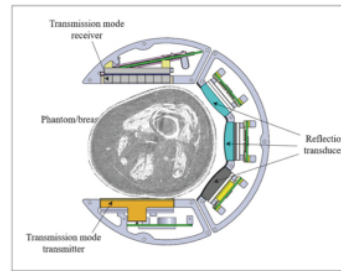
Schematic of rotating ultrasound transmitter
